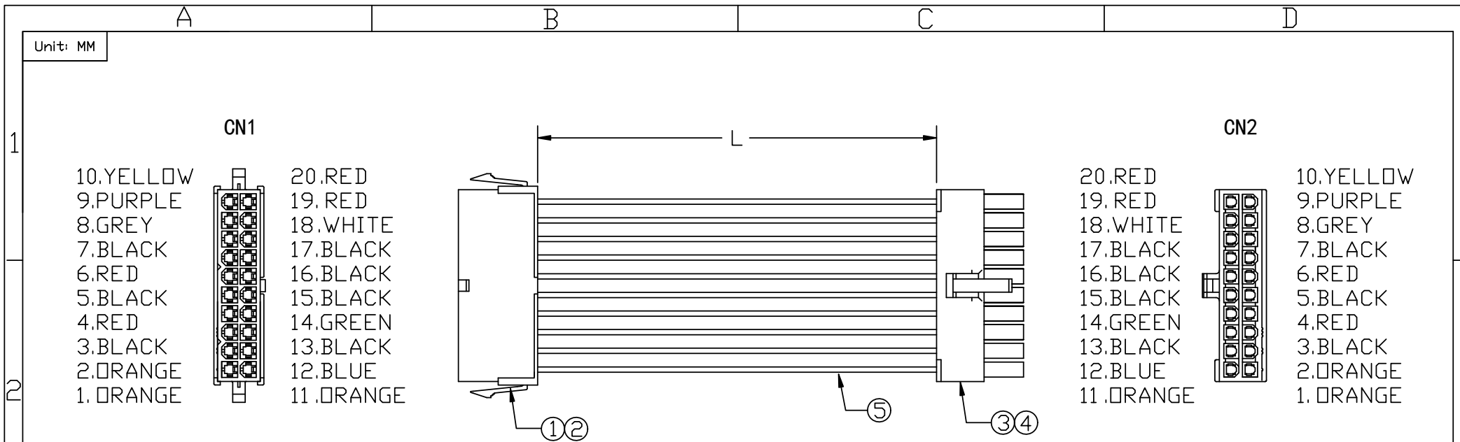
Connection table
